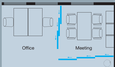
Triple running and guide track for extremely space-saving solutions.
